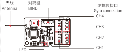
GMr Receiver interface diagram:
